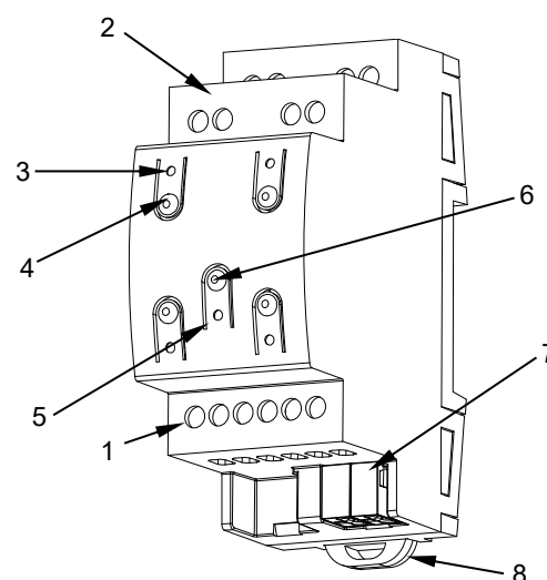
Figure 1: MINiBOX 45 v3
