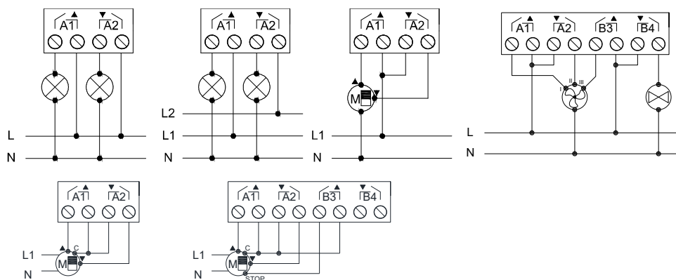
Figure 3: Wiring example (from left to right): 2 loads, 2 loads connected to different phases, shutter and fan coil, shutter with 2 dry contacts, shutter with 3 dry contacts.
