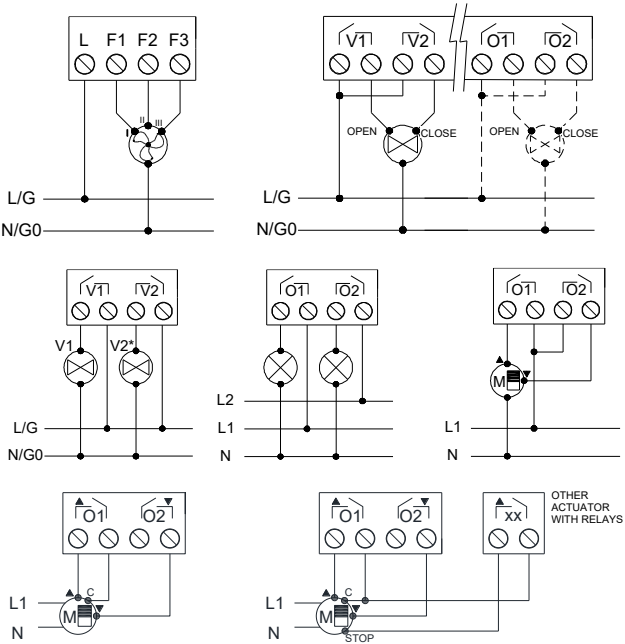
Figure 2: Wiring example (from left to right and from top to bottom): Three-speed fan, 1 or 2 three-point valves, 2 open/close valves, 2 loads connected to different phases, shutter channel, shutter with 2 dry contacts and shutter with 3 dry contacts
