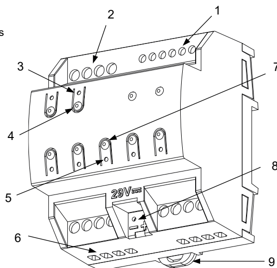
Figure 1: MAXinBOX 66 v3
