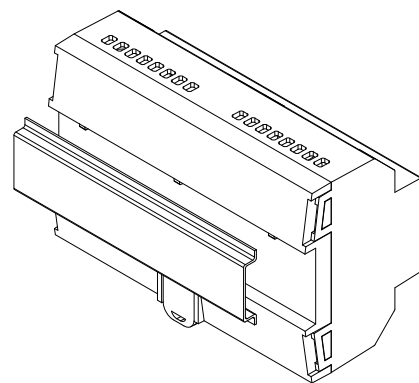
Figure 2: Mounting MAXinBOX 16 v4 on DIN rail
