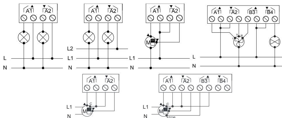
Figure 3: Wiring example (from left to right and up to down): 2 loads, 2 loads connected to different phases, shutter, fan coil, shutter with 2 dry contacts, shutter with 3 dry contacts.
