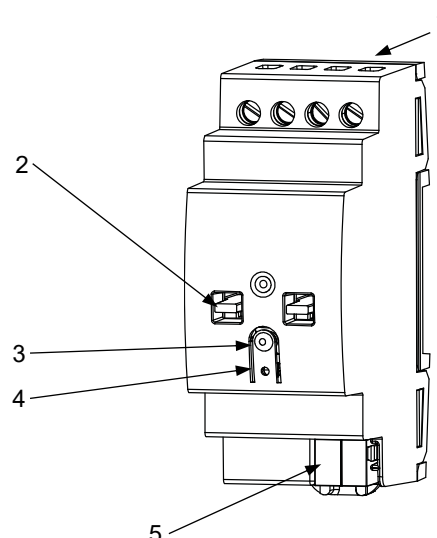
Figure 1: IndustrialBOX Current 2
