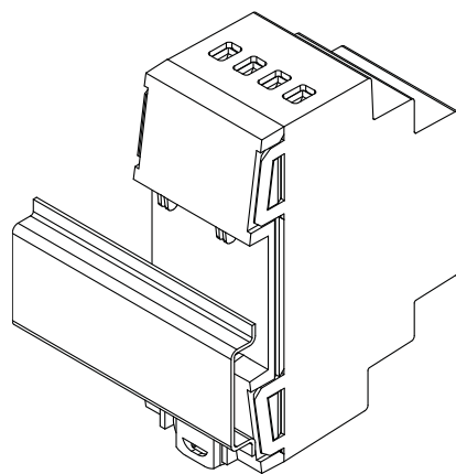
Figure 3: Mounting IndustrialBOX Current 2 on DIN rail
