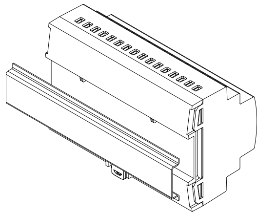
Figure 3: Mounting IndustrialBOX 8 on DIN rail
