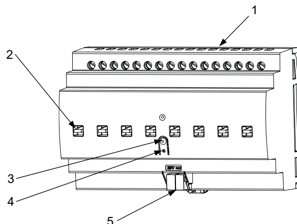
Figure 1: IndustrialBOX 8
