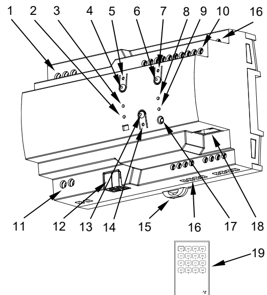
Figure 1: ALLinBOX 88 v2
